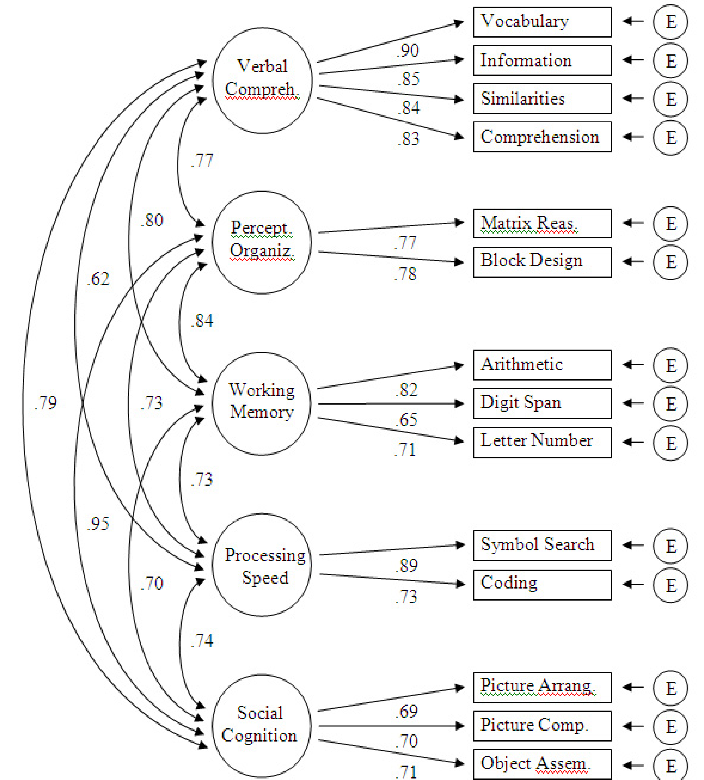
Figure 1. Model M5:PA,PC,OA. Best fitting model for 14 subtests.
